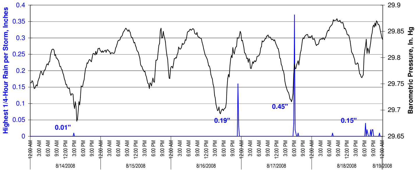
Chart 6: Pine Home Station, Monsoon 8/14-8/18 2008
